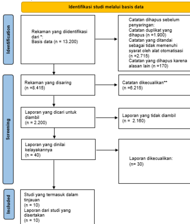
Gambar 1. Diagram PRISMA
